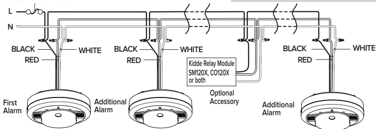
Figure 9-B, Interconnect Wiring Diagram
