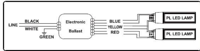
Retrofit luminaire with 2 lamps
