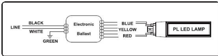
Retrofit luminaire with 1 lamp
