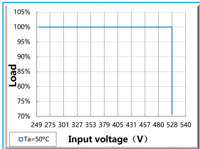
◇ Derating curve
