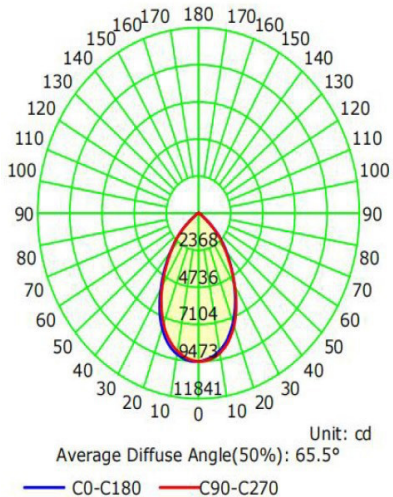
Luminous Intensity Distribution Curve
