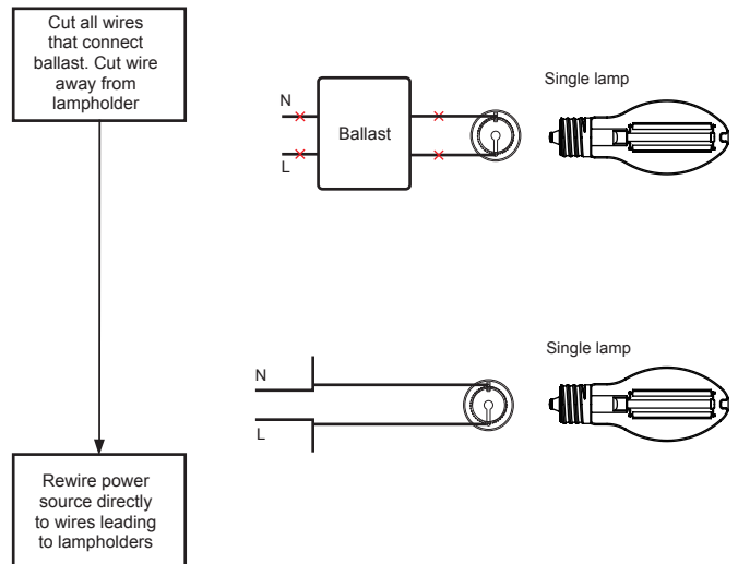
Diagram 2 – Electronic ballast fixture wiring modification
