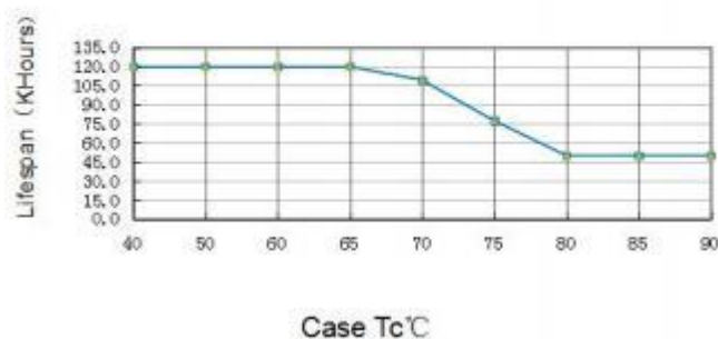
Lifespan VS Case Tc°C
