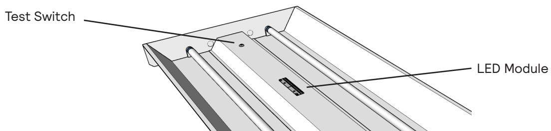
Figure 6. Completed Luminaire
