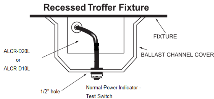
Illustration 1: Integral (No Flex) Mounting ALCR-D20L & ALCR-D10L
