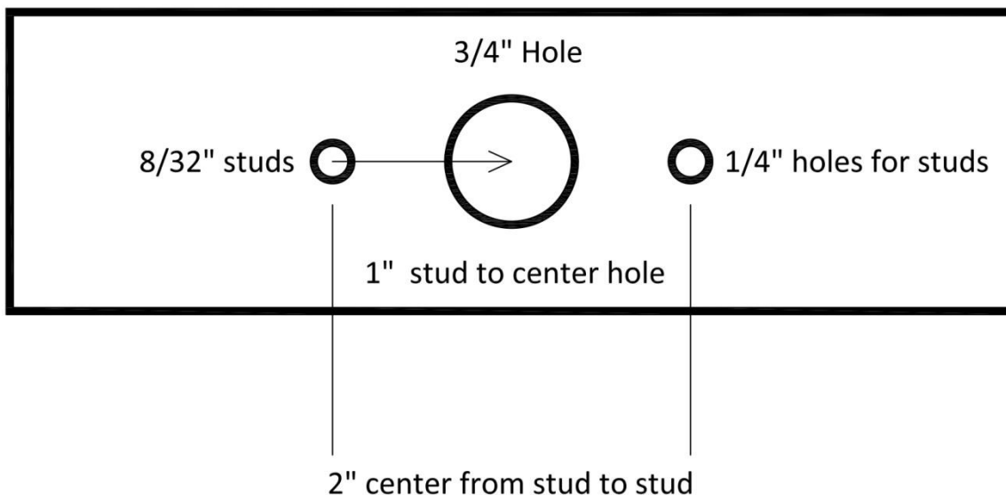
Stud Mounting Detail
