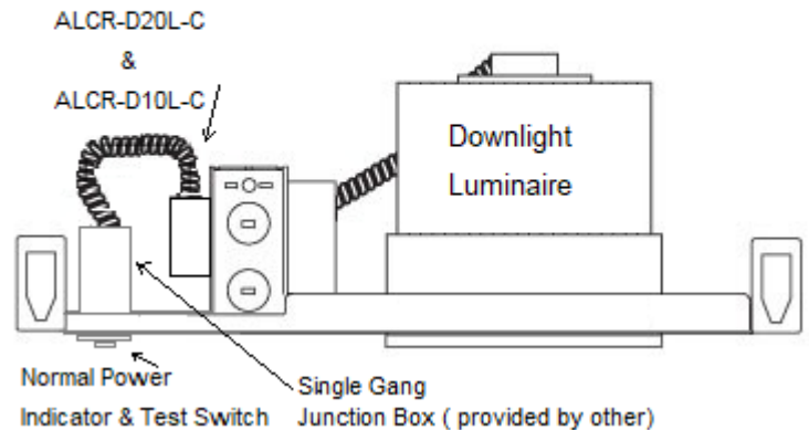
Illustration 2: ALCR-D20L-C & ALCR-D10L-C Stud Mounting with single flex (Bottom Mount)
