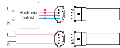
Bypass electronic ballasts to replace 2G7/2GX7 4-pin CFL PL lamps
