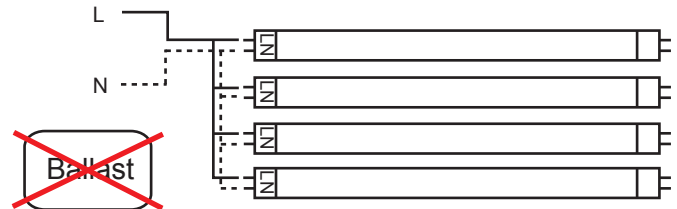
Diagram 4 – Multiple tube wiring
