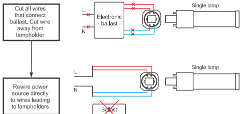
Diagram 2 – Electronic ballast fixture wiring modification
