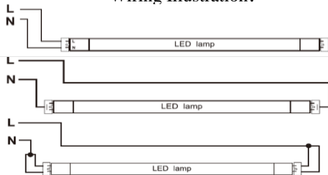
Wiring Illustration:
