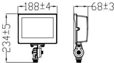
Knuckle
