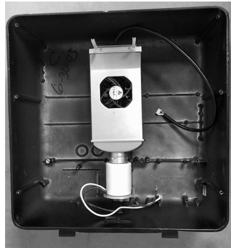
Figure 2 – Ballast bypassed and removed, LED retrofit driver installed with support legs
