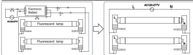
Retrofit luminaire with non-shunted lampholders — 2 lamps
