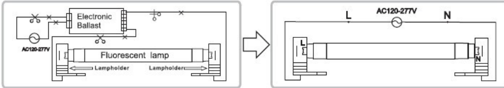
Retrofit luminaire with shunted lampholders — 1 lamp
