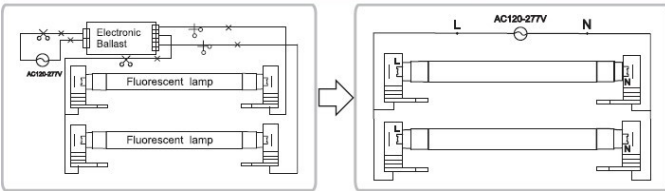
Retrofit luminaire with shunted lampholders — 2 lamps
