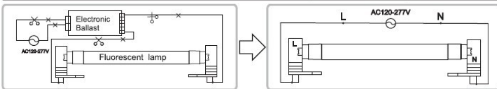
Retrofit luminaire with non-shunted lampholders — 1 lamp
