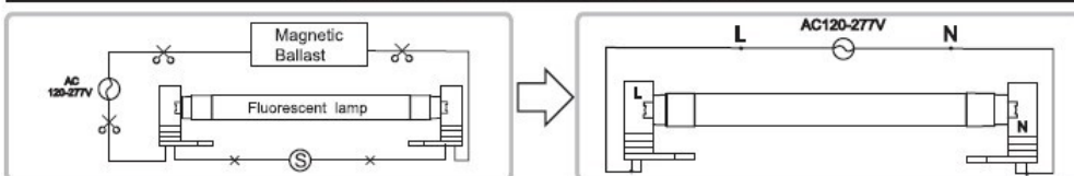
Retrofit luminaire Magnetic Ballast
