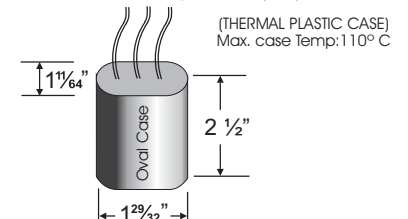
IGNITOR 37-63-AS-9.1-N7 Ballast to Lamp Distance (BTL): 2 feet
