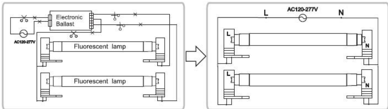
Retrofit Luminaire with Non-shunted Lampholders - 2 Lamps
