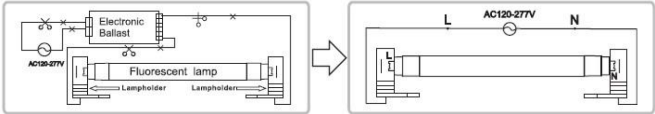
Retrofit Luminaire with Shunted Lampholders - 2 Lamps
