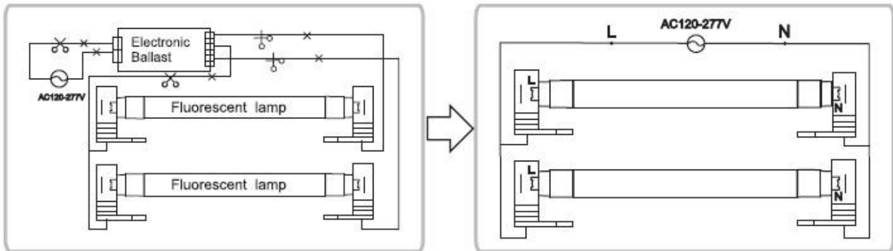
Retrofit Luminaire with Non-shunted Lampholders - 1 Lamp
