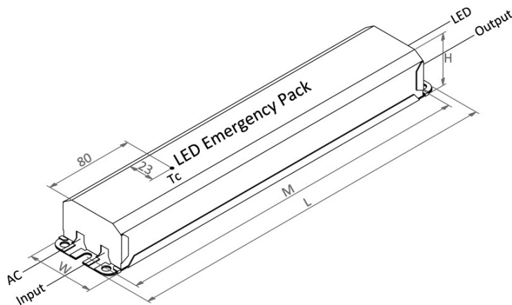
20/25W Emergency Driver
