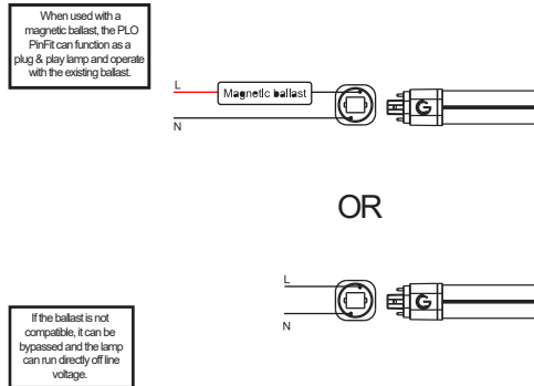
Diagram 3 - 2 pins mode - Magnetic ballast or BYPass installation wiring
