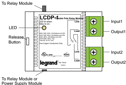
Fig. 4: Relay for DPST Loads
