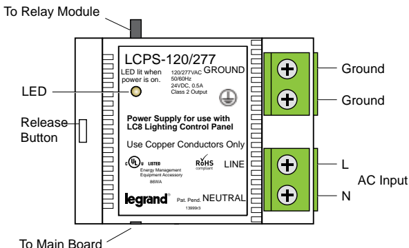
Fig. 2: Power Supply
