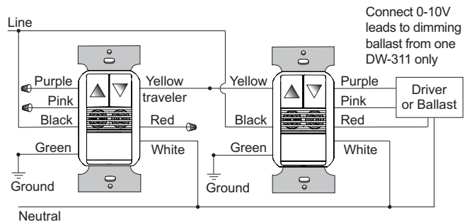
Multi-way wiring
