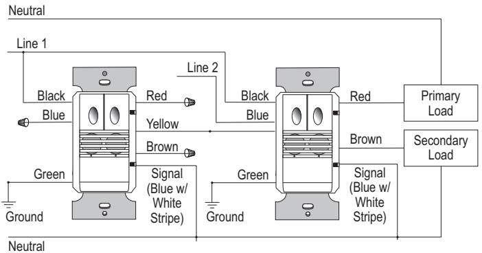
Two-phase Wiring
