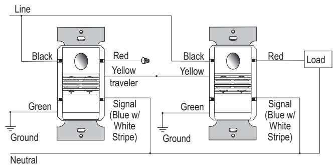
Typical Wiring (DSW-301 up to 4 sensors)
