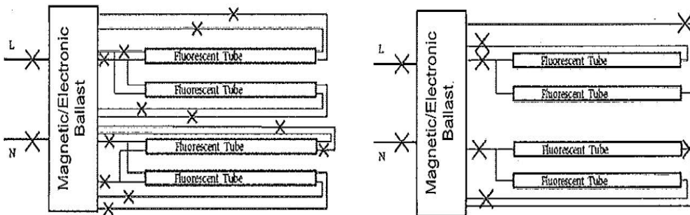
Fig. 4 (Removing Magnetic/Electronic Ballast)
