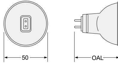
Base: GU5.3
