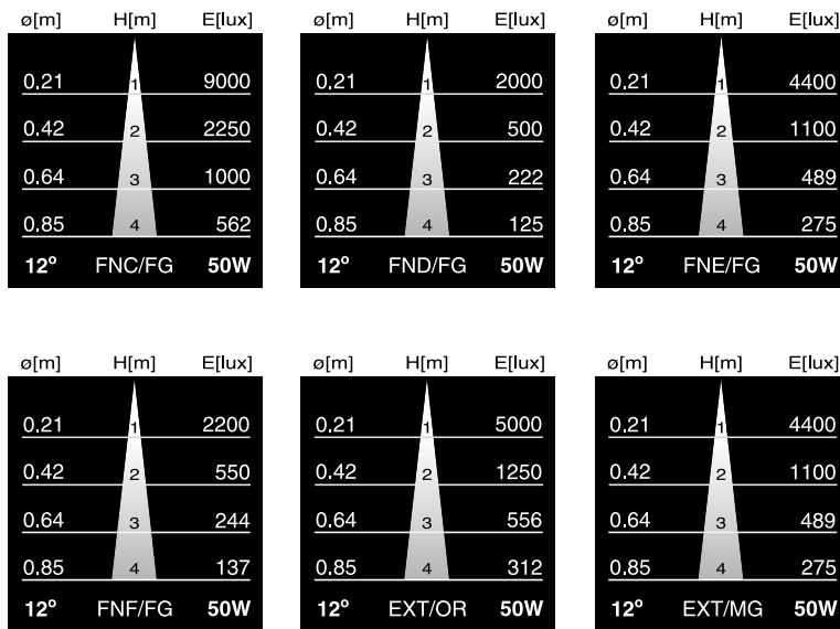
Base: GU5.3
