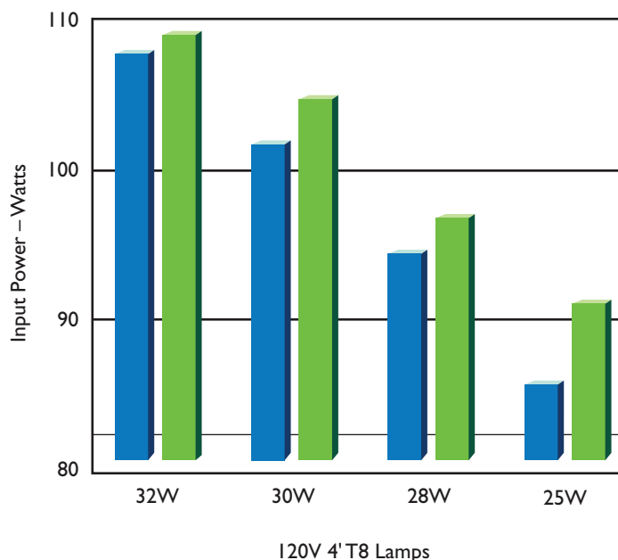
Current-Fed vs. Voltage-Fed Ballasts What's the difference?
