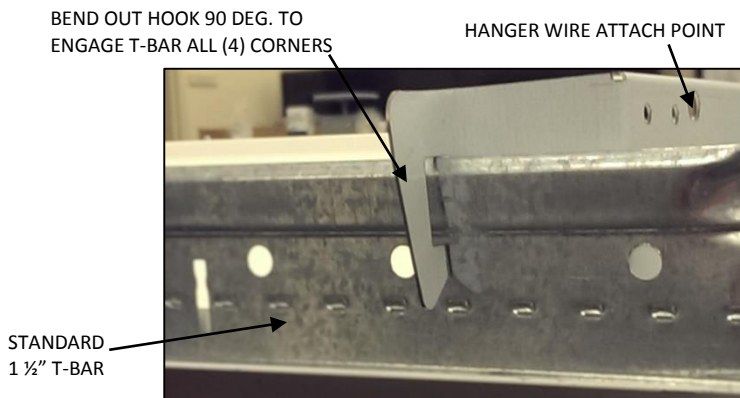
Figure 1: Built In T-Bar Clip
