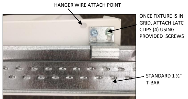
Figure 2: LATC Installation (ORDERABLE OPTION)
