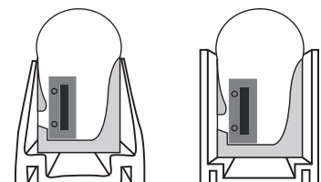
Cut-view when used with track (sold separately)
