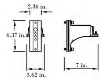
Mounting Arm
