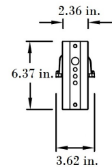
Mounting Arm
