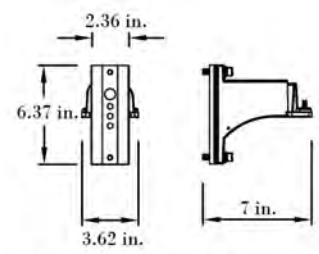
Mounting Arm
