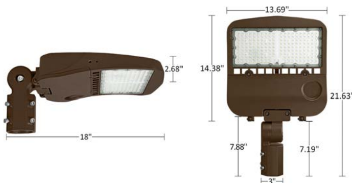
Mounting Dimensions:
