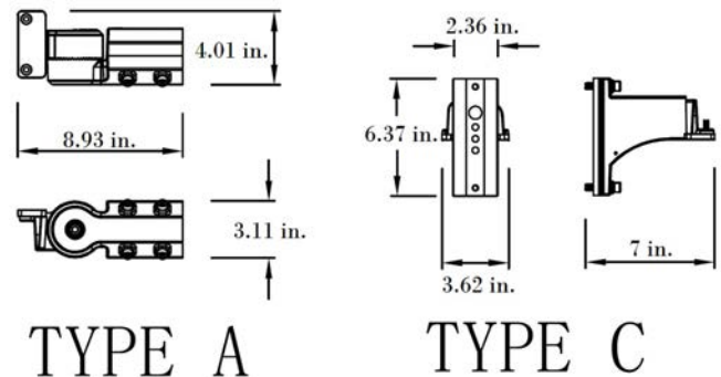
Mounting Dimensions:
