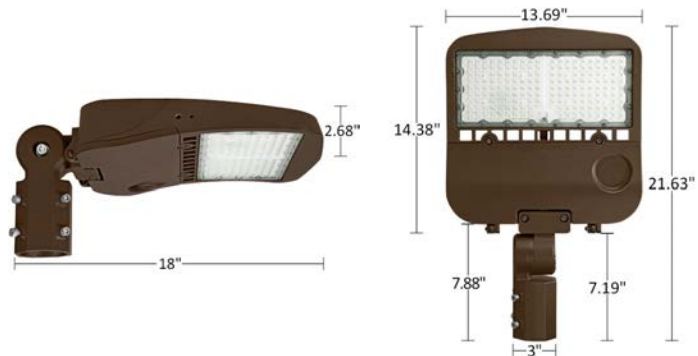
Mounting Dimensions:
