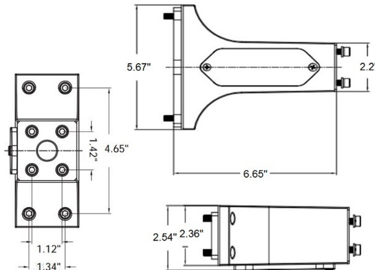
Mounting Arm for Square Pole
