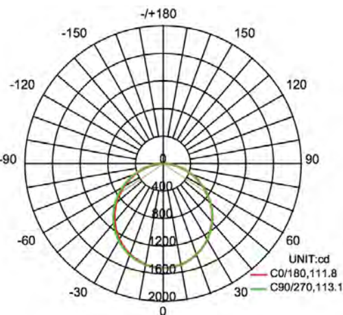
AVERAGE BEAM ANGLE(50%):112.4 DEG
