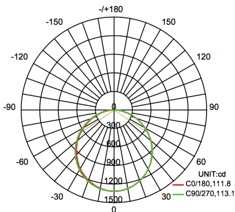
AVERAGE BEAM ANGLE(50%):112.5 DEG
