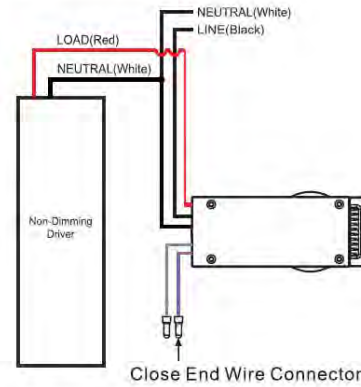
BRI823-B-D wiring with non-dimming ballast or LED driver. Non-Dimming Driver
