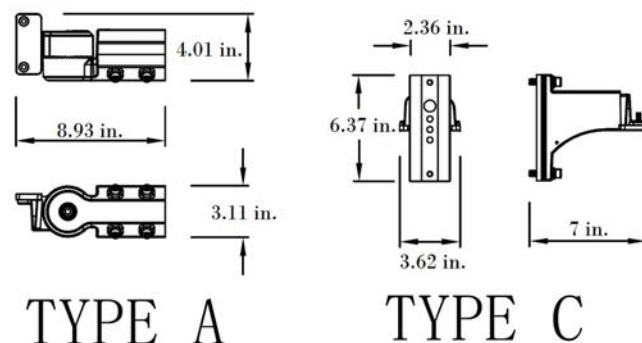
Mounting Dimensions:
