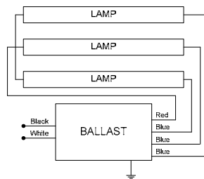
For 3-lamp, 2-lamp and 1-lamp application individually cap red and blue leads
