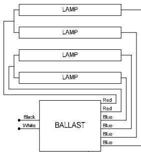
For 3-lamp, 2-lamp and 1-lamp application individually cap red and blue leads
