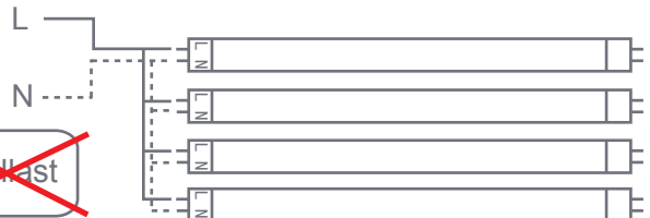
Diagram 4 – Multiple tube wiring
