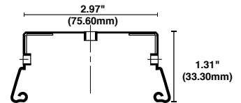
Mounting assembly-LVTH4CL/MA
