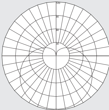
Maximum Candela = 118 Located At Horizontal Angle = 67.5, Vertical Angle = 2.5 Vertical Plane Through Horizontal Angles (90 - 80)
