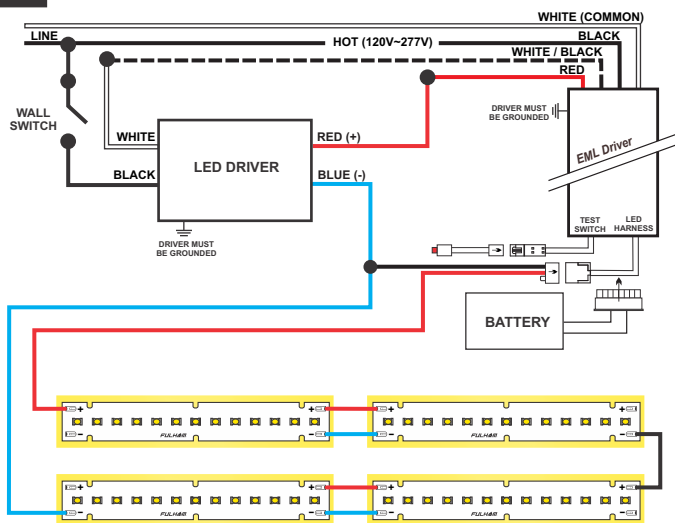
28-B Series / Parallel, Four (4) Modules, Two (4) Emergency
