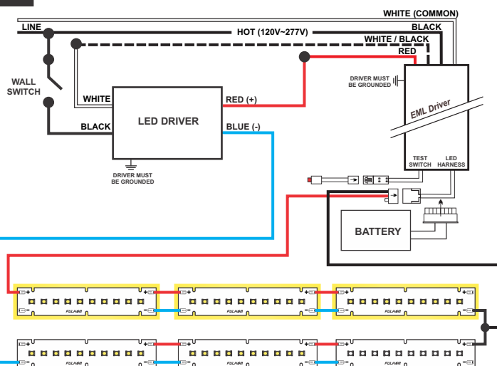
30-B Series / Parallel, Six (6) Modules, Three (3) Emergency
