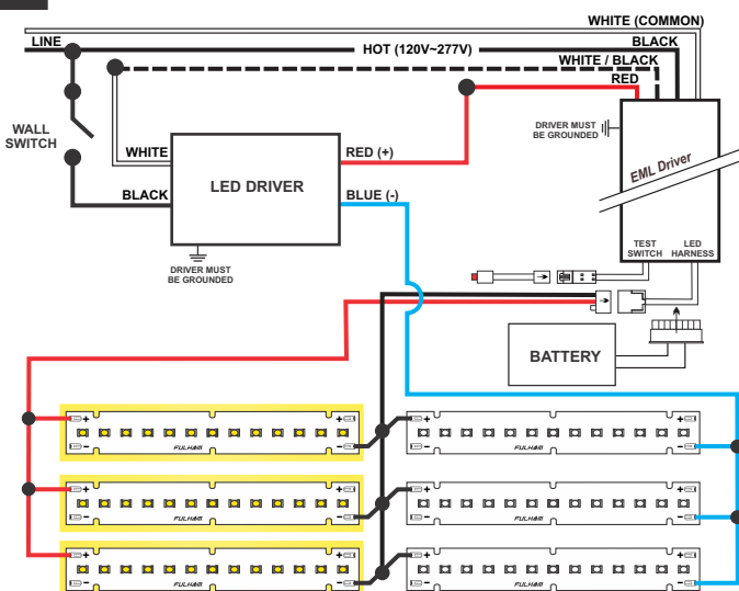
30-A Series / Parallel, Six (6) Modules, Three (3) in Emergency
