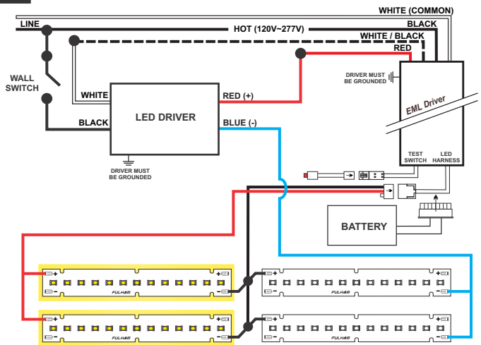
27-A Series / Parallel, Four (4) Modules, Two (2) Emergency
