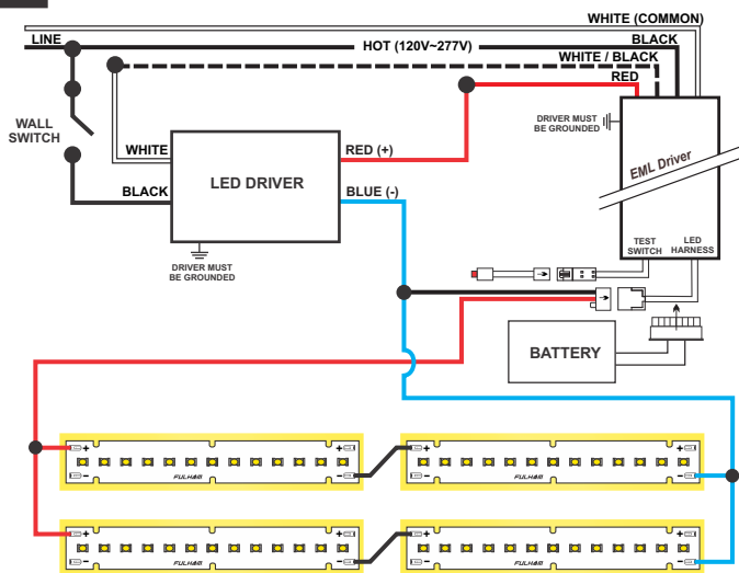
28-A Series / Parallel, Four (4) Modules, Two (4) Emergency
