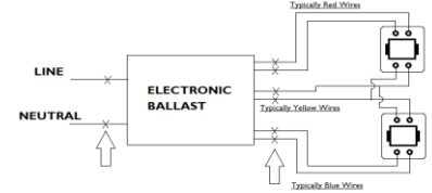
Wiring Diagram - 4 PIN Ballast Bypass. Two Lamp.
