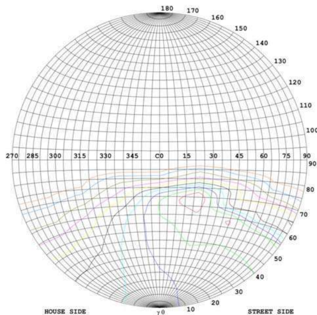
ISOCANDELA DIAGRAM
