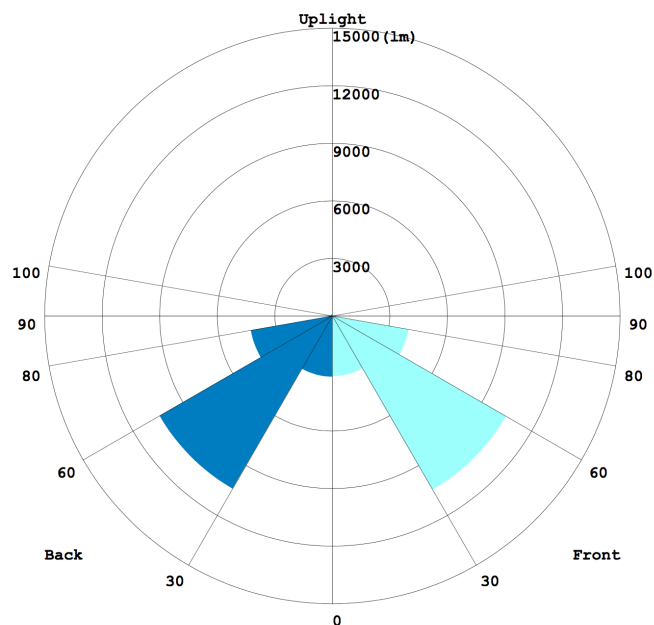
LUMINAIRE CLASSIFICATION SYSTEM (LCS) GRAPH
