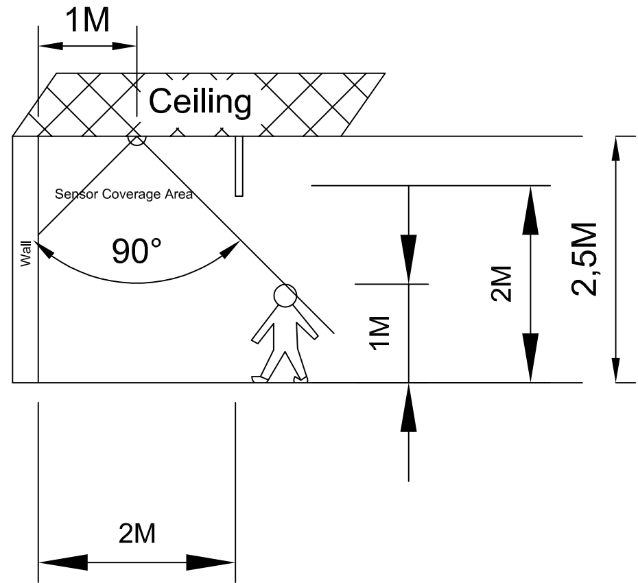
Ceiling Mount
