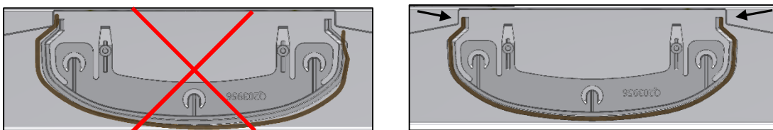
Figure 4: Cross section of lens installed onto fixture
