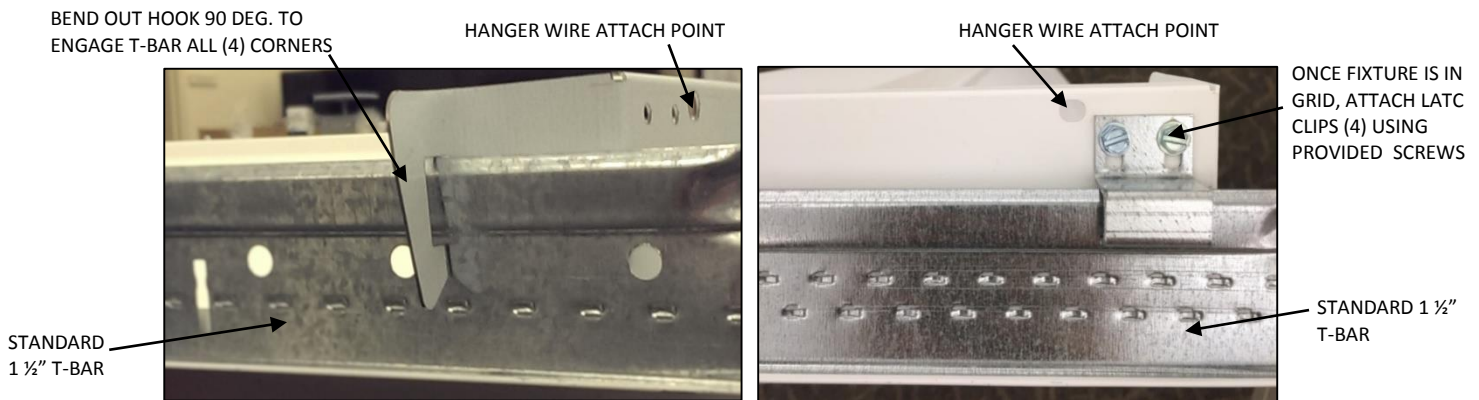
Figure 1: Built In T-Bar Clip
