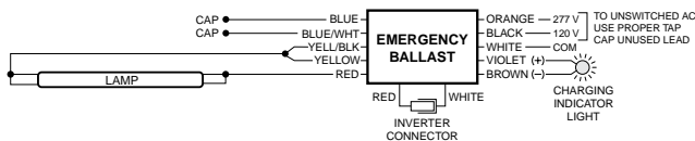
FIG I ONE (1) 17-215 W LAMP WITHOUT AC BALLAST
