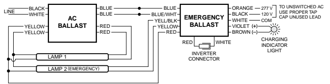
FIG D TWO (2) LAMP RAPID START BALLAST
