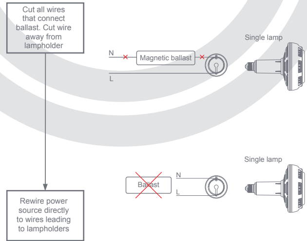
Diagram 3 – Magnetic ballast fixture wiring modification
